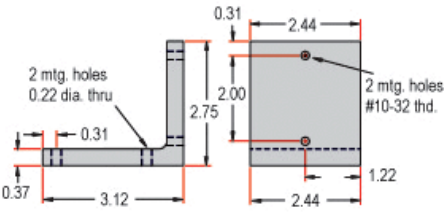
2.62" Z-Axis Adapter Plate (#54-378)
