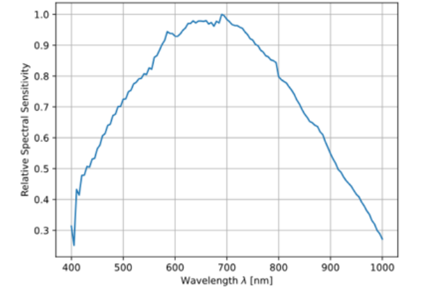
IMX900 Sensor QE Curve
