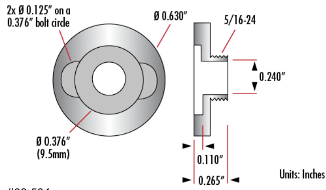
Pinhole Adapter for Stage Type B, #38-534
