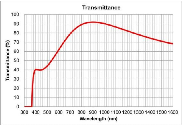
LCPLN20XIR Transmission Graph
