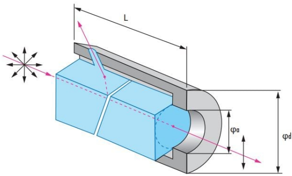
Glan-Laser Polarizers
