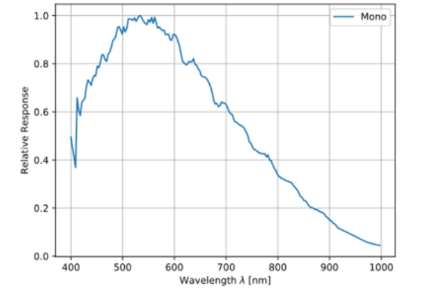
GMAX2505 Sensor QE Curve
