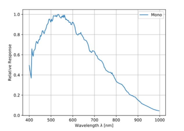
GMAX2505 Sensor QE Curve
