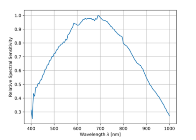
IMX900 Sensor QE Curve
