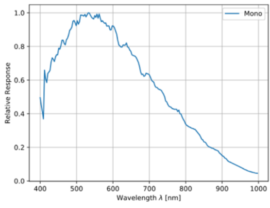
GMAX2509 Sensor QE Curve
