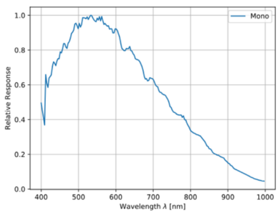
GMAX2518 Sensor QE Curve
