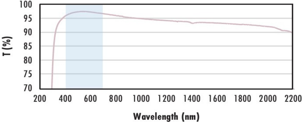
N-BK7 with VIS-EXT Coating Typical Transmission
