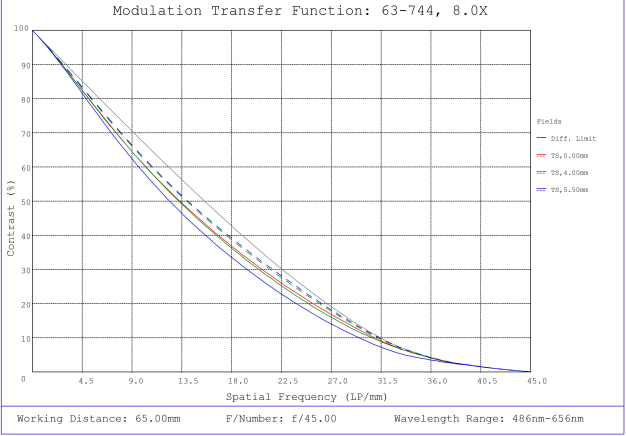
#63-744, 8X, 65mm WD CompactTL™ Telecentric Lens, Modulated Transfer Function (MTF) Plot, 65mm Working Distance, f45
