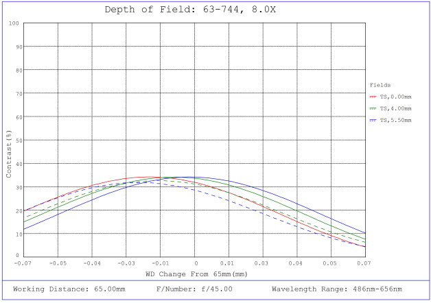
#63-744, 8X, 65mm WD CompactTL™ Telecentric Lens, Depth of Field Plot, 65mm Working Distance, f45
