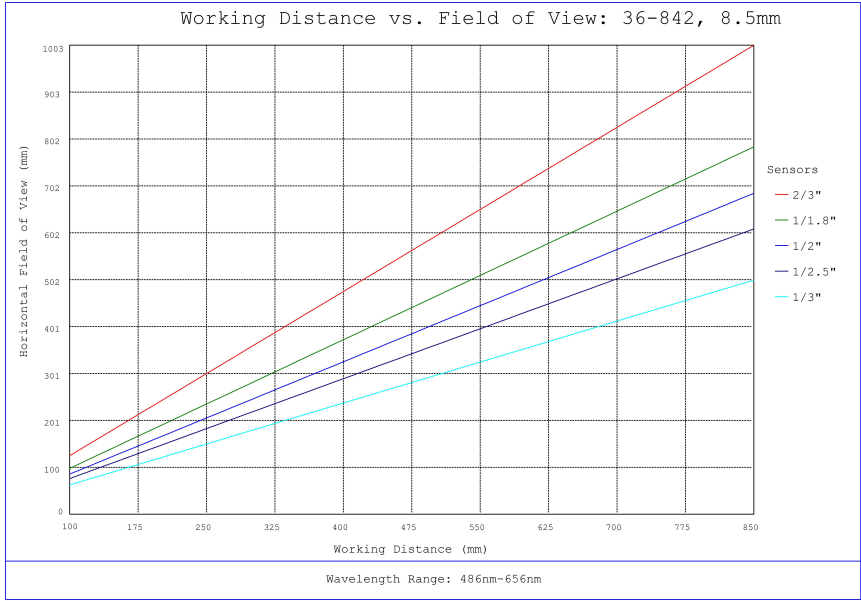
#36-842, 8.5mm, f/5.6 Cr Series Fixed Focal Length Lens, Working Distance versus Field of View Plot
