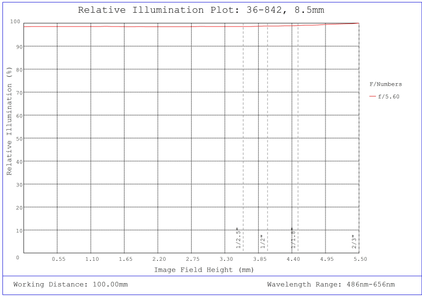
#36-842, 8.5mm, f/5.6 Cr Series Fixed Focal Length Lens, Relative Illumination Plot
