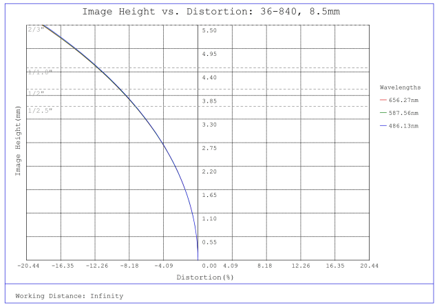
#36-840, 8.5mm, f/2.8 Cr Series Fixed Focal Length Lens, Distortion Plot
