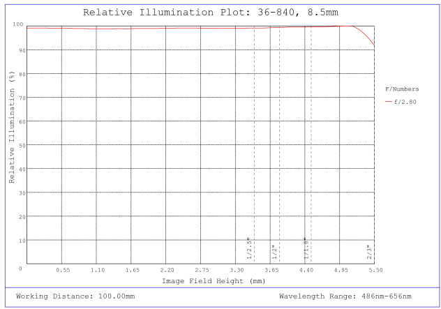
#36-840, 8.5mm, f/2.8 Cr Series Fixed Focal Length Lens, Relative Illumination Plot
