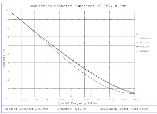
#36-754, 8.5mm f/16, 75mm-∞ Primary WD, HRi Series Fixed Focal Length Lens, Modulated Transfer Function (MTF) Plot, 200mm Working Distance, f16
