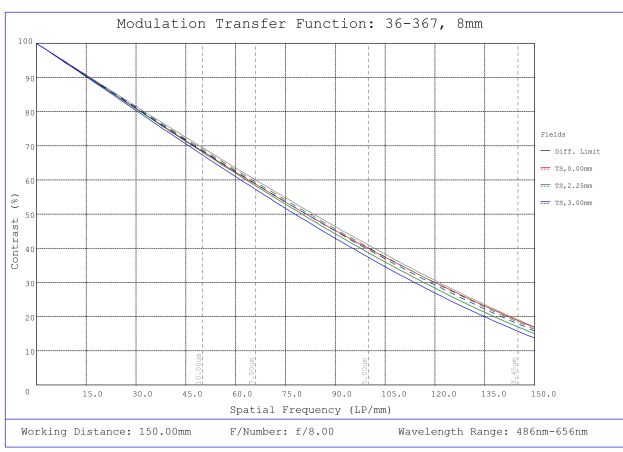
#36-367, 8.0mm FL f/8 Rugged Blue Series M12 Lens, Modulated Transfer Function (MTF) Plot, 150mm Working Distance, f8
