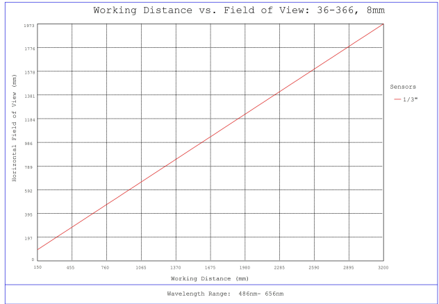
#36-366, 8.0mm FL f/5.6 Rugged Blue Series M12 Lens, Working Distance versus Field of View Plot
