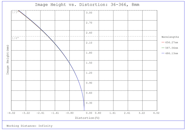
#36-366, 8.0mm FL f/5.6 Rugged Blue Series M12 Lens, Distortion Plot
