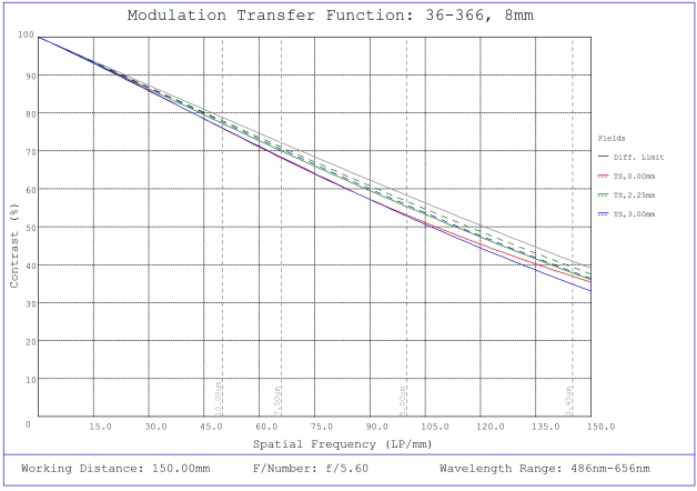
#36-366, 8.0mm FL f/5.6 Rugged Blue Series M12 Lens, Modulated Transfer Function (MTF) Plot, 150mm Working Distance, f5.6
