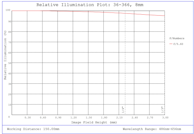
#36-366, 8.0mm FL f/5.6 Rugged Blue Series M12 Lens, Relative Illumination Plot
