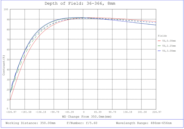
#36-366, 8.0mm FL f/5.6 Rugged Blue Series M12 Lens, Depth of Field Plot, 350mm Working Distance, f5.6
