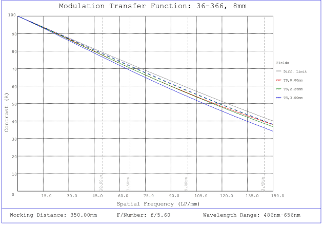
#36-366, 8.0mm FL f/5.6 Rugged Blue Series M12 Lens, Modulated Transfer Function (MTF) Plot, 350mm Working Distance, f5.6
