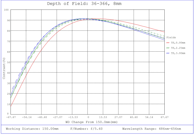
#36-366, 8.0mm FL f/5.6 Rugged Blue Series M12 Lens, Depth of Field Plot, 150mm Working Distance, f5.6
