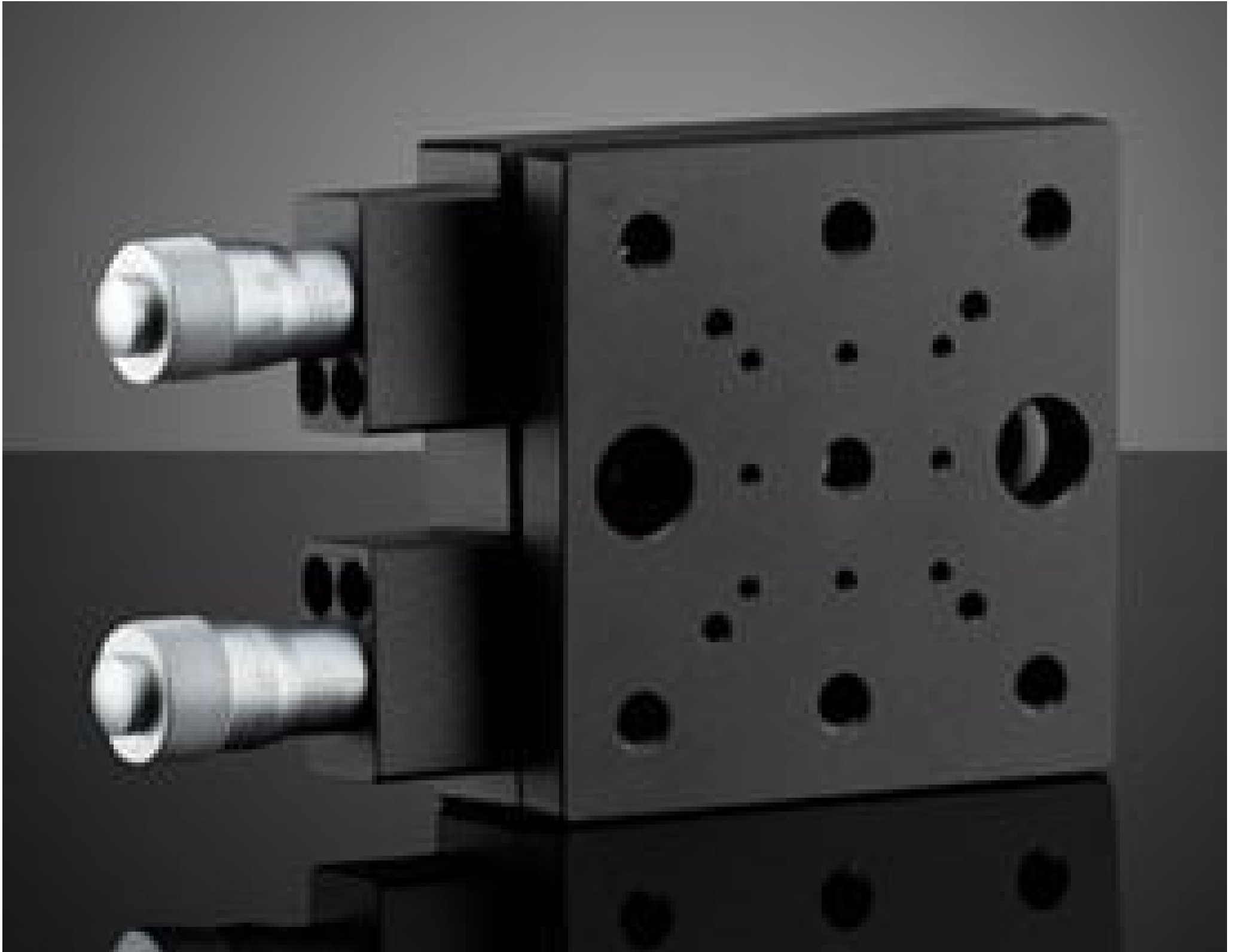
70mm Micrometer Tilt Stage
