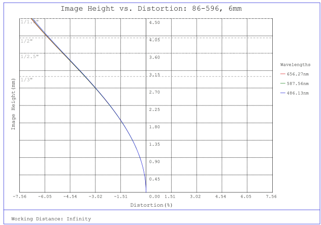
#86-596, 6mm, f/8 Ci Series Fixed Focal Length Lens, Distortion Plot
