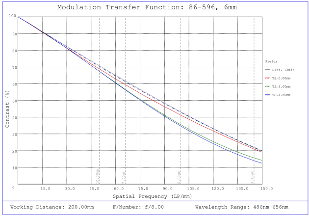
#86-596, 6mm, f/8 Ci Series Fixed Focal Length Lens, Modulated Transfer Function (MTF) Plot, 200mm Working Distance, f8
