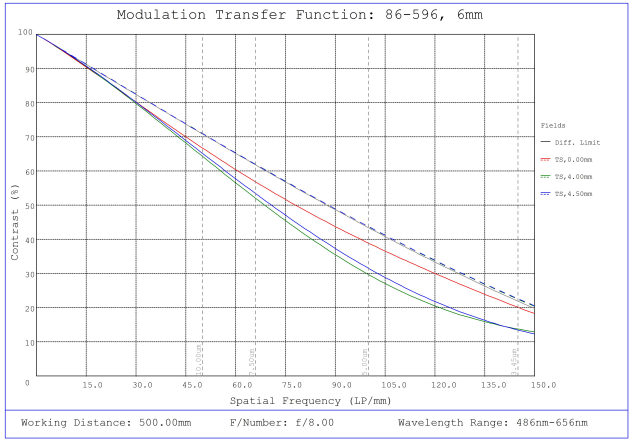
#86-596, 6mm, f/8 Ci Series Fixed Focal Length Lens, Modulated Transfer Function (MTF) Plot, 500mm Working Distance, f8
