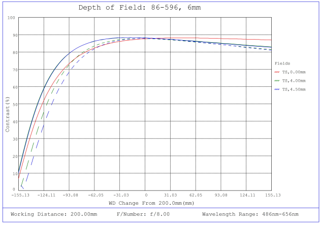
#86-596, 6mm, f/8 Ci Series Fixed Focal Length Lens, Depth of Field Plot, 200mm Working Distance, f8
