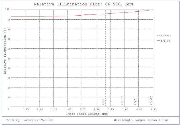
#86-596, 6mm, f/8 Ci Series Fixed Focal Length Lens, Relative Illumination Plot
