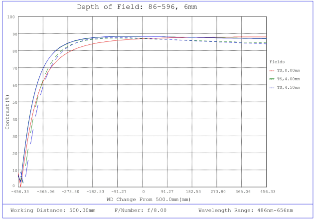
#86-596, 6mm, f/8 Ci Series Fixed Focal Length Lens, Depth of Field Plot, 500mm Working Distance, f8
