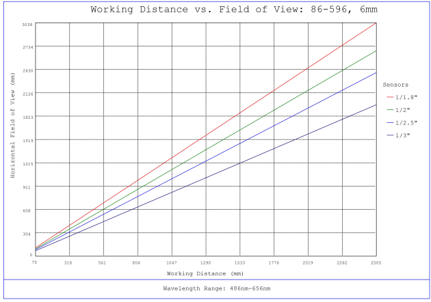
#86-596, 6mm, f/8 Ci Series Fixed Focal Length Lens, Working Distance versus Field of View Plot
