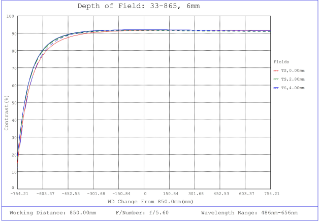
#33-865, 6mm, f/5.6 UCi Series Fixed Focal Length Lens, Depth of Field Plot, 850mm Working Distance, f5.6
