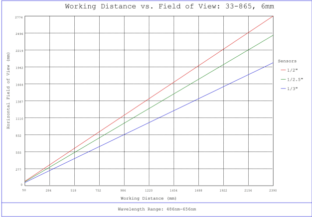
#33-865, 6mm, f/5.6 UCi Series Fixed Focal Length Lens, Working Distance versus Field of View Plot
