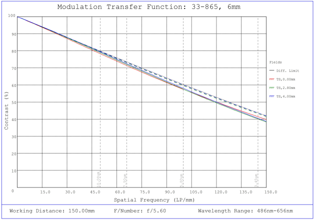
#33-865, 6mm, f/5.6 UCi Series Fixed Focal Length Lens, Modulated Transfer Function (MTF) Plot, 150mm Working Distance, f5.6
