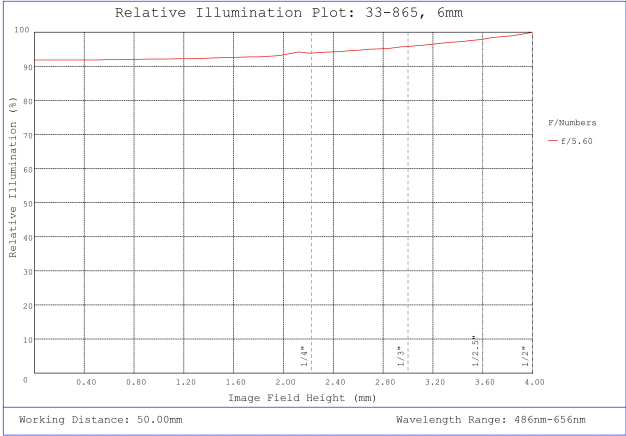
#33-865, 6mm, f/5.6 UCi Series Fixed Focal Length Lens, Relative Illumination Plot
