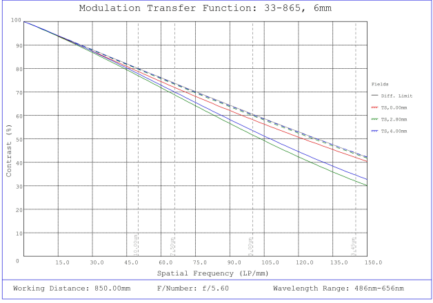
#33-865, 6mm, f/5.6 UCi Series Fixed Focal Length Lens, Modulated Transfer Function (MTF) Plot, 850mm Working Distance, f5.6
