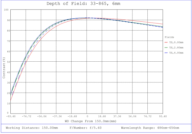
#33-865, 6mm, f/5.6 UCi Series Fixed Focal Length Lens, Depth of Field Plot, 150mm Working Distance, f5.6
