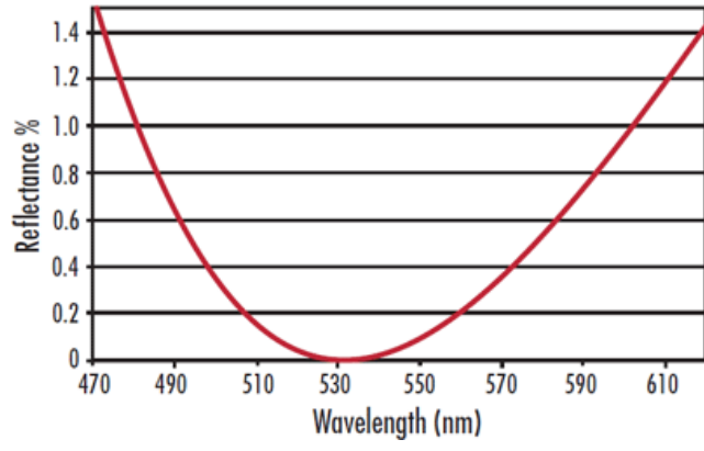
532nm V-Coat R_{(obs)} < 0.25\% @ 532\text{nm}
