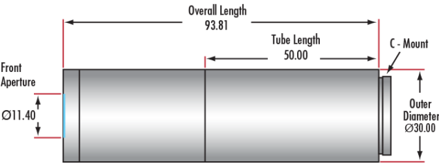
5X Compact Adjustable Objective (#88-353, #34-767)
