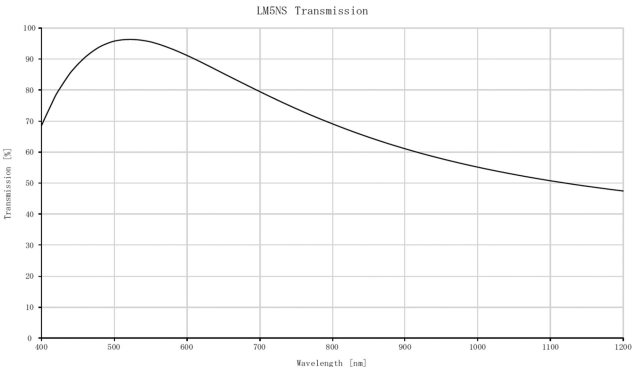
5mm FL, f/4, Low Distortion M12 Lens, Transmission Plot
