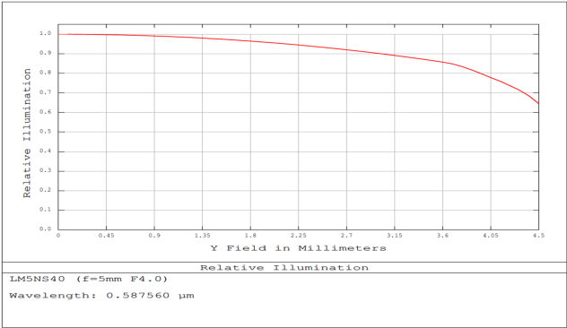
5mm FL, f/4, Low Distortion M12 Lens, Relative Illumination Plot
