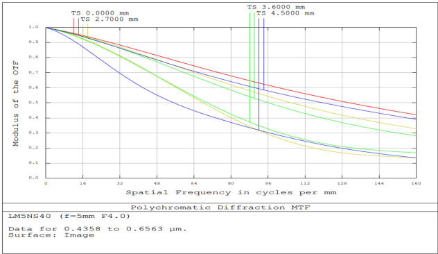
5mm FL, f/4, Low Distortion M12 Lens, MTF Plot
