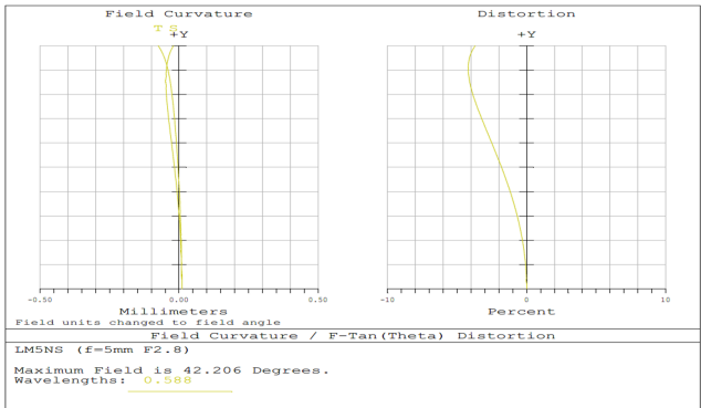
5mm FL, f/4, Low Distortion M12 Lens, Distribution Plot
