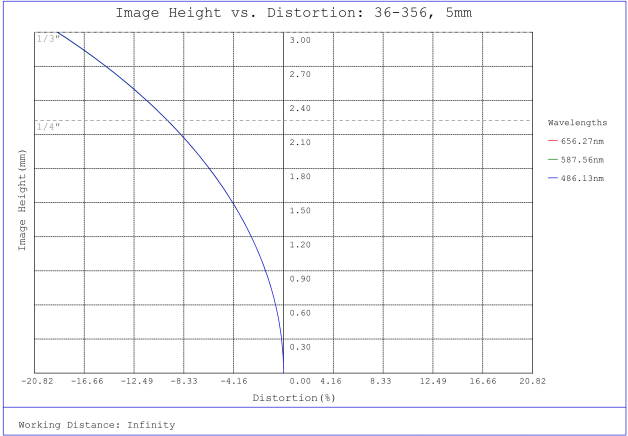
#36-356, 5mm FL f/2.5, Rugged Blue Series M12 Lens, Distortion Plot
