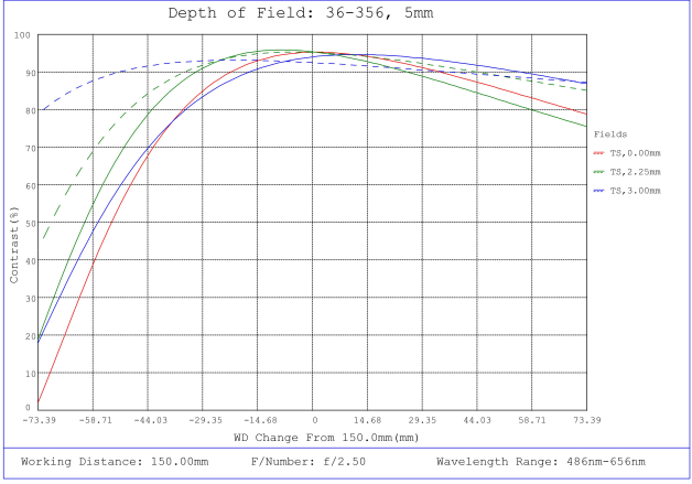
#36-356, 5mm FL f/2.5, Rugged Blue Series M12 Lens, Depth of Field Plot, 150mm Working Distance, f2.5
