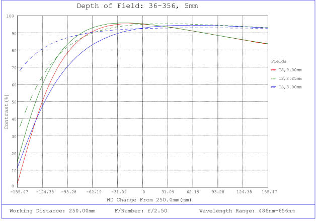
#36-356, 5mm FL f/2.5, Rugged Blue Series M12 Lens, Depth of Field Plot, 250mm Working Distance, f2.5
