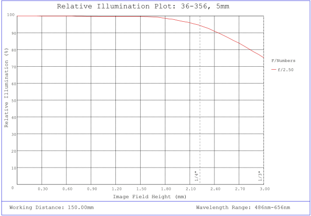
#36-356, 5mm FL f/2.5, Rugged Blue Series M12 Lens, Relative Illumination Plot
