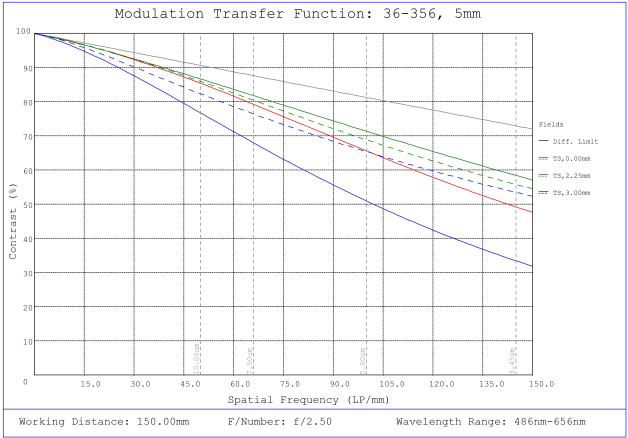
#36-356, 5mm FL f/2.5, Rugged Blue Series M12 Lens, Modulated Transfer Function (MTF) Plot, 150mm Working Distance, f2.5
