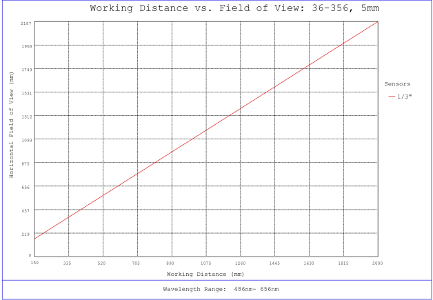
#36-356, 5mm FL f/2.5, Rugged Blue Series M12 Lens, Working Distance versus Field of View Plot
