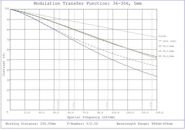
#36-356, 5mm FL f/2.5, Rugged Blue Series M12 Lens, Modulated Transfer Function (MTF) Plot, 250mm Working Distance, f2.5
