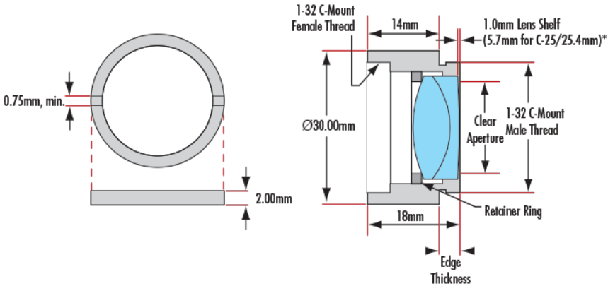
C-Thread Achromat / Thick Lens Mount
