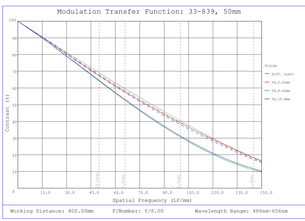
#33-839, 50mm f/8.0, HPI Series Fixed Focal Length Lens, Modulated Transfer Function (MTF) Plot, 400mm Working Distance, f8
