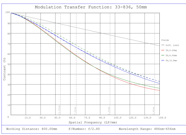
#33-836, 50mm f/2.8, HPI Series Fixed Focal Length Lens, Modulated Transfer Function (MTF) Plot, 400mm Working Distance, f2.8
