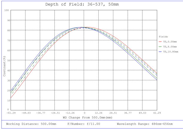
#36-537, 50mm f/11, HPr Series Fixed Focal Length Lens, Depth of Field Plot, 500mm Working Distance, f11
