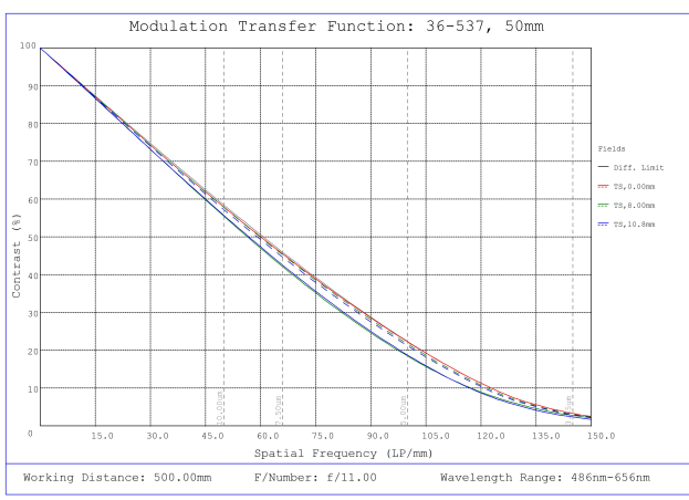
#36-537, 50mm f/11, HPr Series Fixed Focal Length Lens, Modulated Transfer Function (MTF) Plot, 500mm Working Distance, f11
