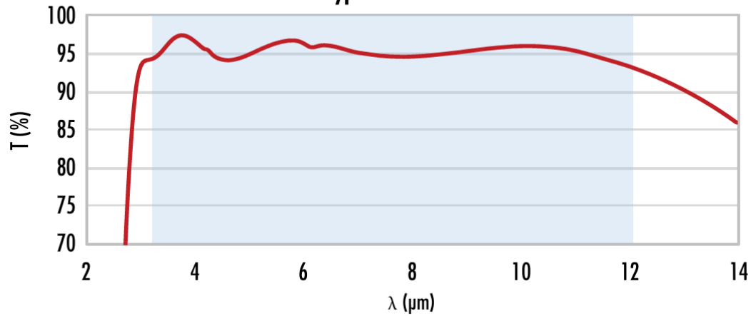
ZnSe with 3-12μm AR Coating Typical Transmission
