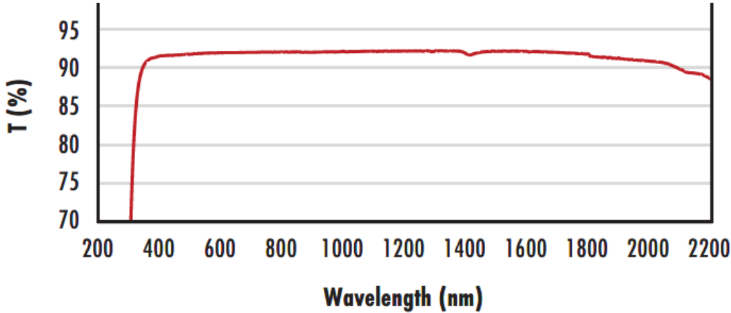
N-BK7 with MgF 2 Coating Typical Transmission
