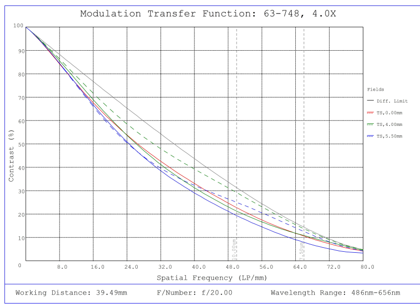
#63-748, 4X, 40mm WD CompactTL™ Telecentric Lens, Modulated Transfer Function (MTF) Plot, 39mm Working Distance, f20
