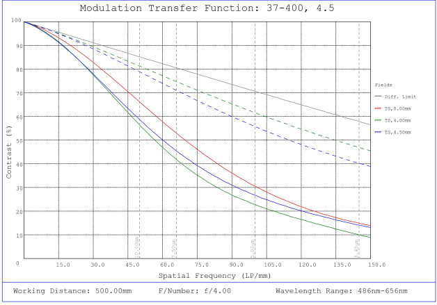
#37-400, 4.5mm, f/4 Cr Series Fixed Focal Length Lens, Modulated Transfer Function (MTF) Plot, 500mm Working Distance, f4
