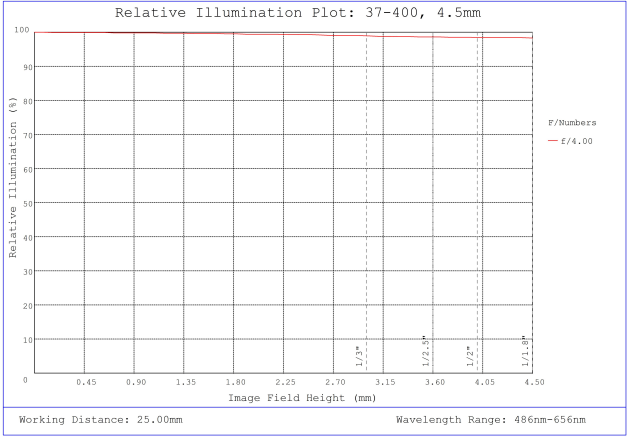
#37-400, 4.5mm, f/4 Cr Series Fixed Focal Length Lens, Relative Illumination Plot
