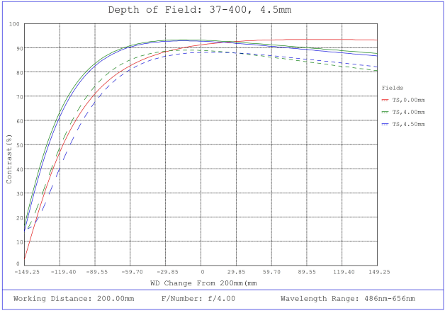
#37-400, 4.5mm, f/4 Cr Series Fixed Focal Length Lens, Depth of Field Plot, 200mm Working Distance, f4
