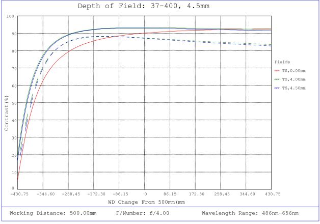
#37-400, 4.5mm, f/4 Cr Series Fixed Focal Length Lens, Depth of Field Plot, 500mm Working Distance, f4
