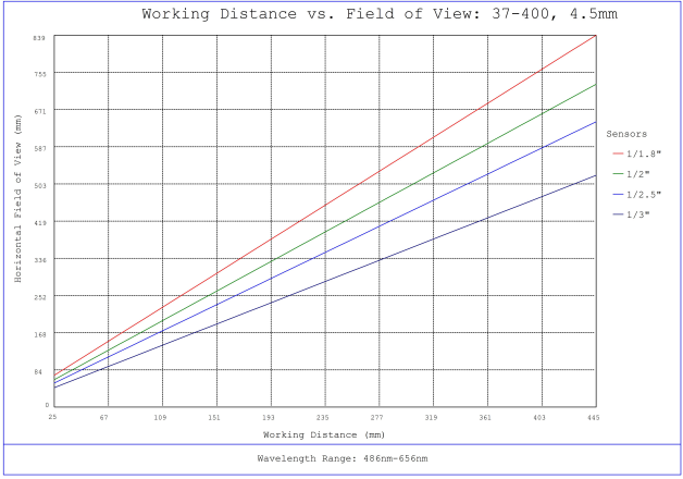
#37-400, 4.5mm, f/4 Cr Series Fixed Focal Length Lens, Working Distance versus Field of View Plot
