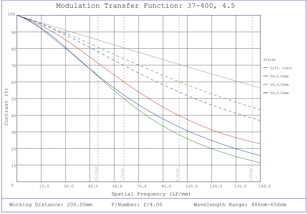
#37-400, 4.5mm, f/4 Cr Series Fixed Focal Length Lens, Modulated Transfer Function (MTF) Plot, 200mm Working Distance, f4
