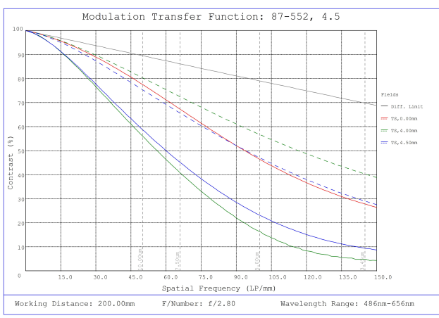
#87-552, 4.5mm, f/2.8 Ci Series Fixed Focal Length Lens, Modulated Transfer Function (MTF) Plot, 200mm Working Distance, f2.8
