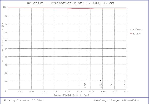
#37-403, 4.5mm, f/11 Cr Series Fixed Focal Length Lens, Relative Illumination Plot
