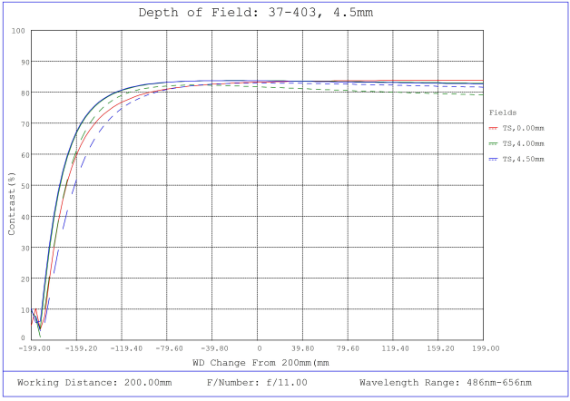
#37-403, 4.5mm, f/11 Cr Series Fixed Focal Length Lens, Depth of Field Plot, 200mm Working Distance, f11
