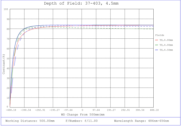
#37-403, 4.5mm, f/11 Cr Series Fixed Focal Length Lens, Depth of Field Plot, 500mm Working Distance, f11
