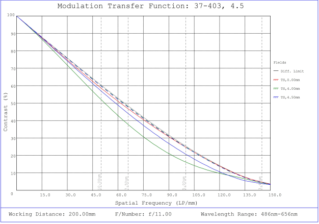
#37-403, 4.5mm, f/11 Cr Series Fixed Focal Length Lens, Modulated Transfer Function (MTF) Plot, 200mm Working Distance, f11
