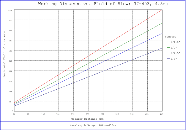
#37-403, 4.5mm, f/11 Cr Series Fixed Focal Length Lens, Working Distance versus Field of View Plot
