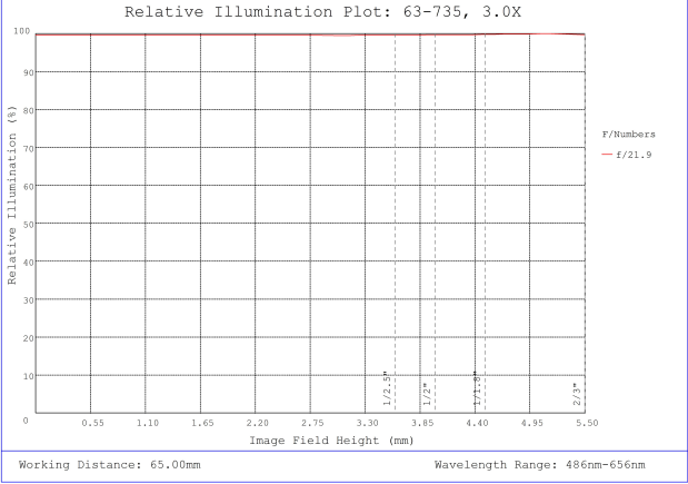
#63-735, 3X, 65mm WD CompactTL™ Telecentric Lens, Relative Illumination Plot
