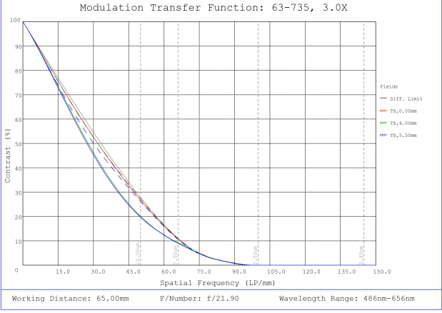
#63-735, 3X, 65mm WD CompactTL™ Telecentric Lens, Modulated Transfer Function (MTF) Plot, 65mm Working Distance, f21.9
