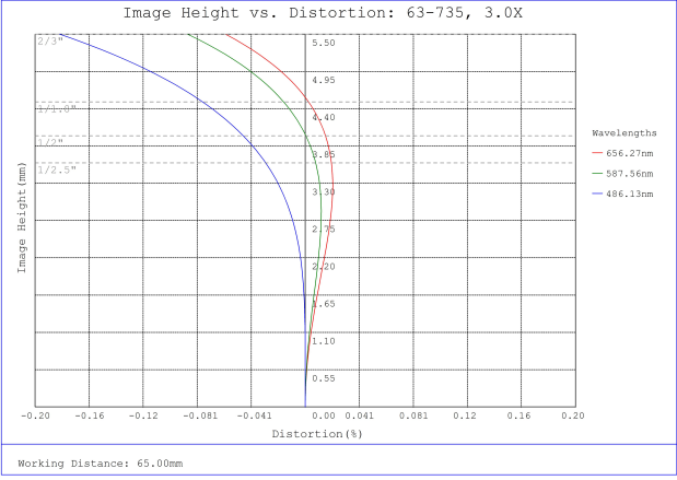
#63-735, 3X, 65mm WD CompactTL™ Telecentric Lens, Distortion Plot
