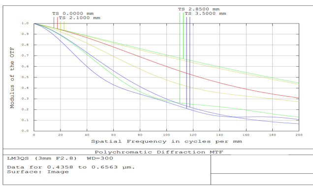
3mm FL, f/4, Low Distortion M12 Lens, MTF Plot
