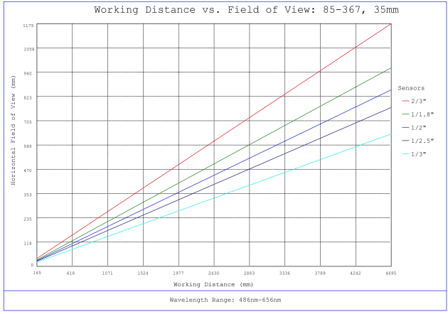
#85-367, 35mm, f/8 Ci Series Fixed Focal Length Lens, Working Distance versus Field of View Plot
