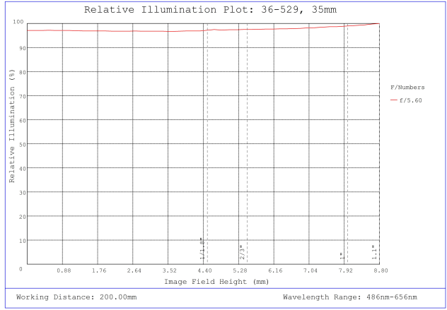
#36-529, 35mm f/5.6, HPr Series Fixed Focal Length Lens, Relative Illumination Plot
