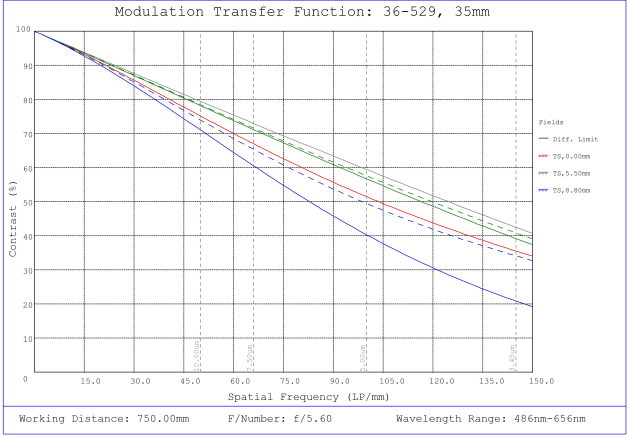
#36-529, 35mm f/5.6, HPr Series Fixed Focal Length Lens, Modulated Transfer Function (MTF) Plot, 750mm Working Distance, f5.6
