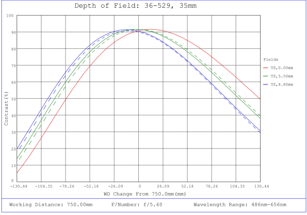
#36-529, 35mm f/5.6, HPr Series Fixed Focal Length Lens, Depth of Field Plot, 750mm Working Distance, f5.6
