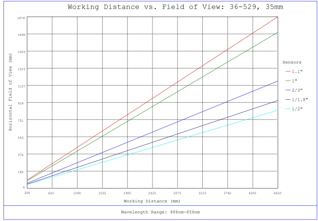
#36-529, 35mm f/5.6, HPr Series Fixed Focal Length Lens, Working Distance versus Field of View Plot
