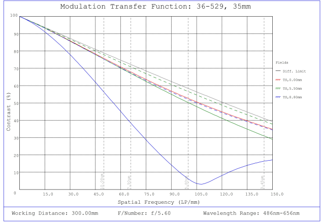
#36-529, 35mm f/5.6, HPr Series Fixed Focal Length Lens, Modulated Transfer Function (MTF) Plot, 300mm Working Distance, f5.6
