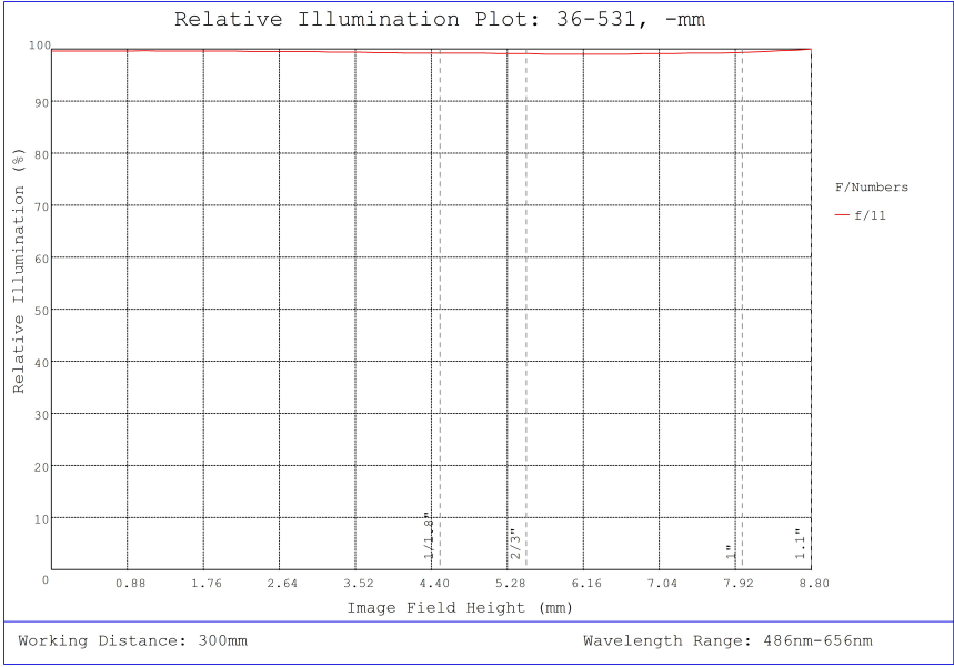
#36-531, 35mm f/11.0, HPr Series Fixed Focal Length Lens, Relative Illumination Plot
