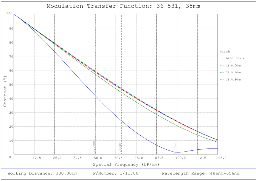
#36-531, 35mm f/11.0, HPr Series Fixed Focal Length Lens, Modulated Transfer Function (MTF) Plot, 300mm Working Distance, f11
