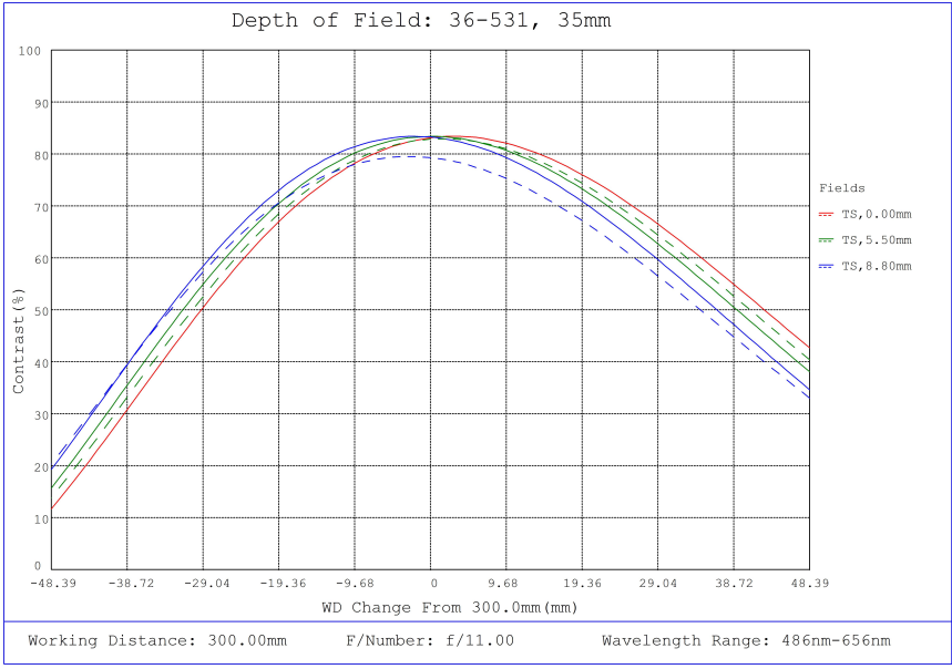
#36-531, 35mm f/11.0, HPr Series Fixed Focal Length Lens, Depth of Field Plot, 300mm Working Distance, f11
