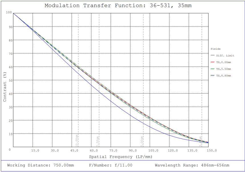
#36-531, 35mm f/11.0, HPr Series Fixed Focal Length Lens, Modulated Transfer Function (MTF) Plot, 750mm Working Distance, f11
