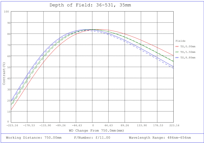
#36-531, 35mm f/11.0, HPr Series Fixed Focal Length Lens, Depth of Field Plot, 750mm Working Distance, f11
