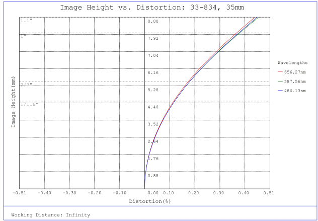
#33-834, 35mm f/11.0, HPI Series Fixed Focal Length Lens, Distortion Plot
