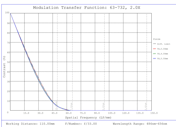
#63-732, 2X, 110mm WD CompactTL™ Telecentric Lens, Modulated Transfer Function (MTF) Plot, 110mm Working Distance, f33
