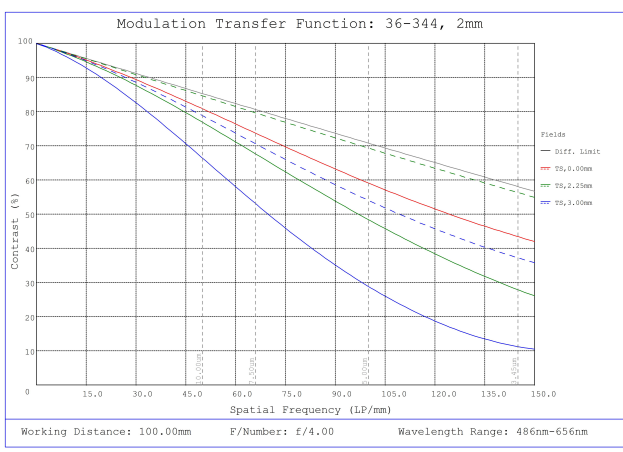
#36-344, 2mm FL f/4 Rugged Blue Series M12 Lens, Modulated Transfer Function (MTF) Plot, 100mm Working Distance, f4
