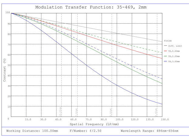
#35-469, 2mm FL f/2.5 IR-Cut Rugged Blue Series M12 Lens, Modulated Transfer Function (MTF) Plot, 100mm Working Distance, f2.5
