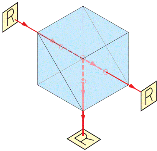
NIR Non-Polarizing Beamsplitters
