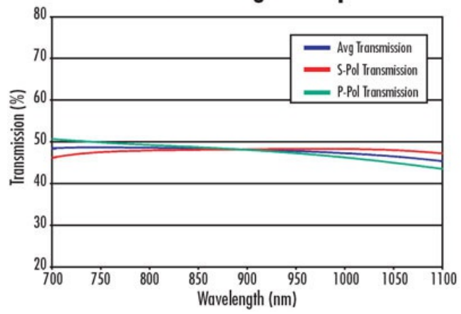
NIR Non-Polarizing Beamsplitters
