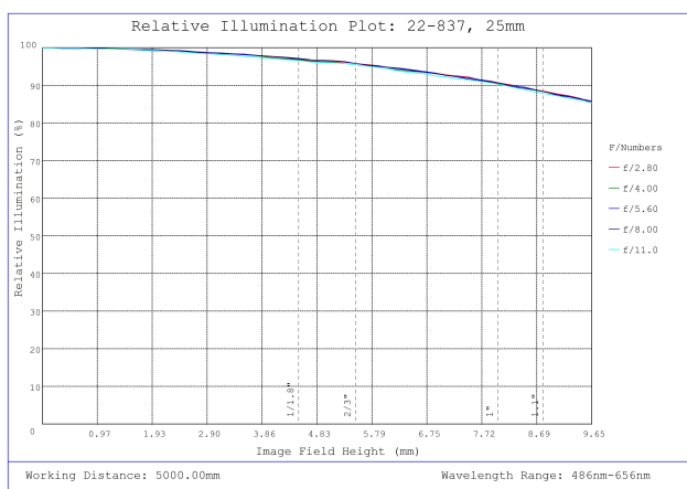
#22-837 - 25mm Focal Length, UAV Series Fixed Focal Length Lenses, Relative Illumination Plot
