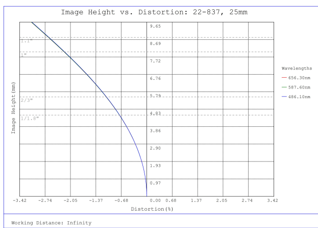
#22-837 - 25mm Focal Length, UAV Series Fixed Focal Length Lenses, Distortion Plot
