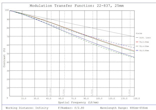
#22-837 - 25mm Focal Length, UAV Series Fixed Focal Length Lenses, Modulated Transfer Function (MTF) Plot, Infinity Working Distance, f2.8
