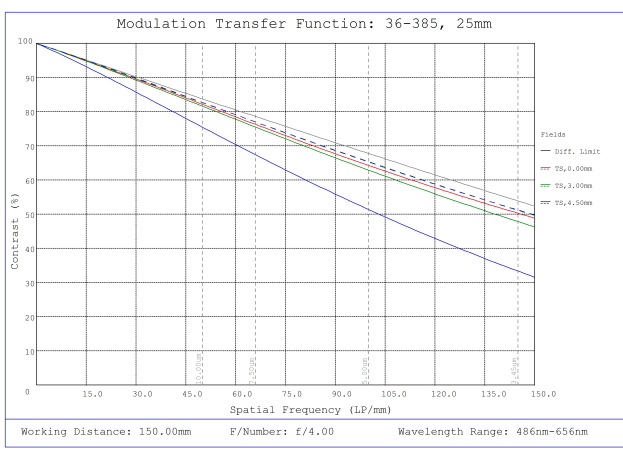
#36-385, 25mm FL f/4, Rugged Blue Series M12 Lens, Modulated Transfer Function (MTF) Plot, 150mm Working Distance, f4
