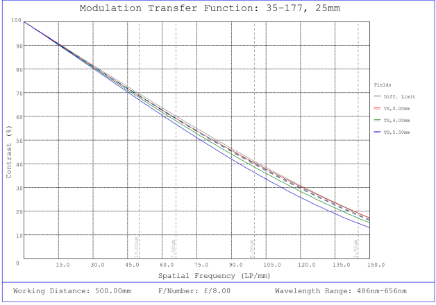
#35-177, 25mm, f/8 Cr Series Fixed Focal Length Lens, Modulated Transfer Function (MTF) Plot, 500mm Working Distance, f8
