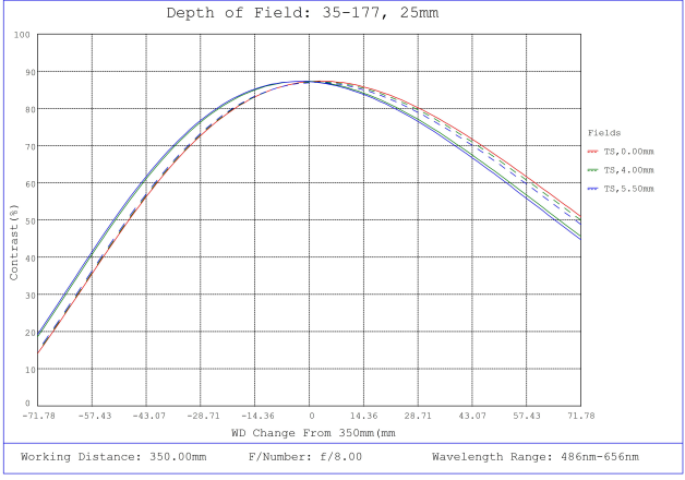
#35-177, 25mm, f/8 Cr Series Fixed Focal Length Lens, Depth of Field Plot, 350mm Working Distance, f8
