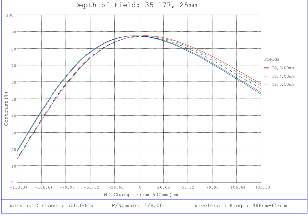
#35-177, 25mm, f/8 Cr Series Fixed Focal Length Lens, Depth of Field Plot, 500mm Working Distance, f8
