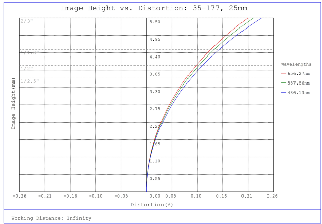
#35-177, 25mm, f/8 Cr Series Fixed Focal Length Lens, Distortion Plot
