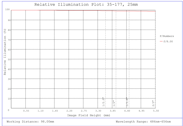
#35-177, 25mm, f/8 Cr Series Fixed Focal Length Lens, Relative Illumination Plot
