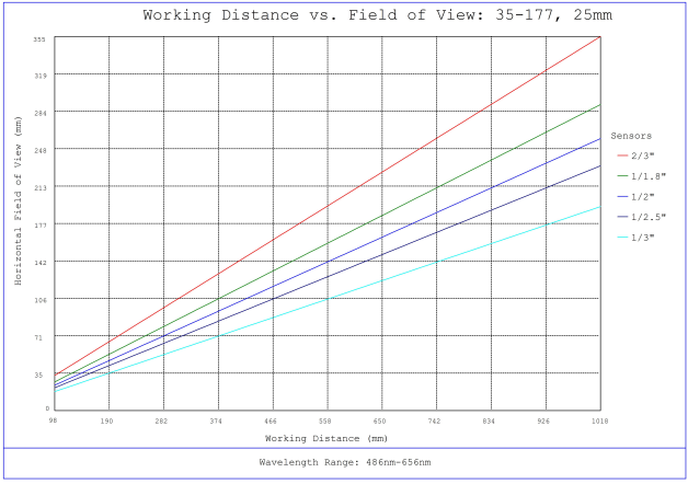
#35-177, 25mm, f/8 Cr Series Fixed Focal Length Lens, Working Distance versus Field of View Plot
