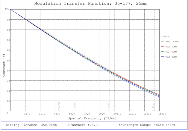
#35-177, 25mm, f/8 Cr Series Fixed Focal Length Lens, Modulated Transfer Function (MTF) Plot, 350mm Working Distance, f8
