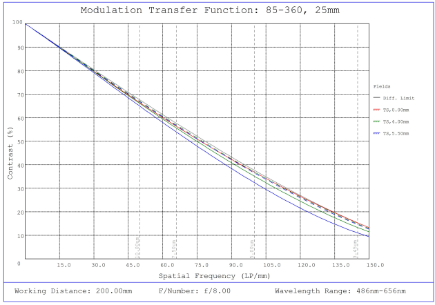
#85-360, 25mm, f/8 Ci Series Fixed Focal Length Lens, Modulated Transfer Function (MTF) Plot, 200mm Working Distance, f8
