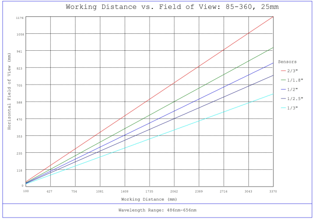
#85-360, 25mm, f/8 Ci Series Fixed Focal Length Lens, Working Distance versus Field of View Plot
