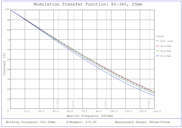
#85-360, 25mm, f/8 Ci Series Fixed Focal Length Lens, Modulated Transfer Function (MTF) Plot, 500mm Working Distance, f8
