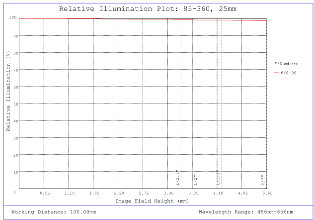
#85-360, 25mm, f/8 Ci Series Fixed Focal Length Lens, Relative Illumination Plot
