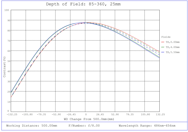
#85-360, 25mm, f/8 Ci Series Fixed Focal Length Lens, Depth of Field Plot, 500mm Working Distance, f8
