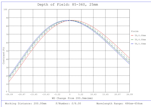
#85-360, 25mm, f/8 Ci Series Fixed Focal Length Lens, Depth of Field Plot, 200mm Working Distance, f8
