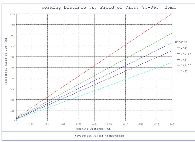
#85-360, 25mm, f/8 Ci Series Fixed Focal Length Lens, Working Distance versus Field of View Plot
