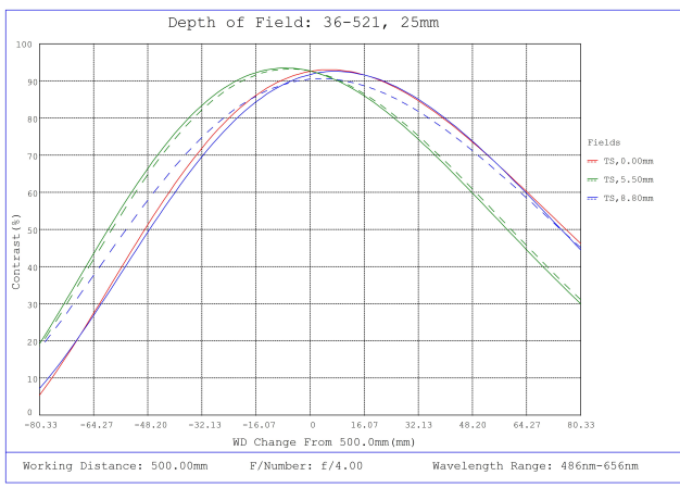
#36-521, 25mm f/4.0, HPr Series Fixed Focal Length Lens, Depth of Field Plot, 500mm Working Distance, f4
