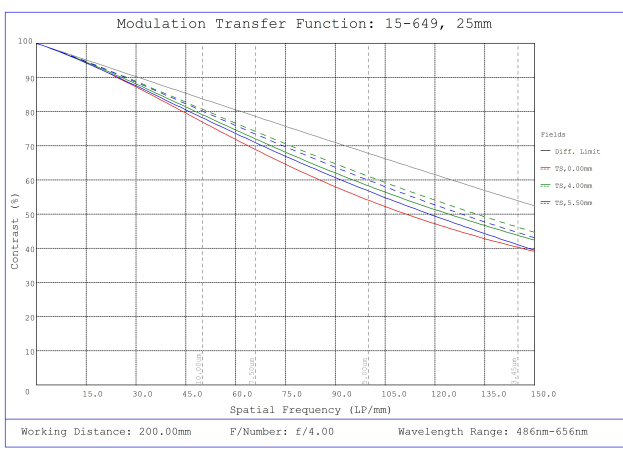
#15-649, 25mm, f/4 Cw Series Fixed Focal Length Lens, Modulated Transfer Function (MTF) Plot, 200mm Working Distance, f4
