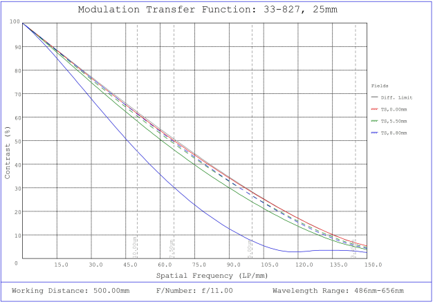
#33-827, 25mm f/11.0, HPi Series Fixed Focal Length Lens, Modulated Transfer Function (MTF) Plot, 500mm Working Distance, f11
